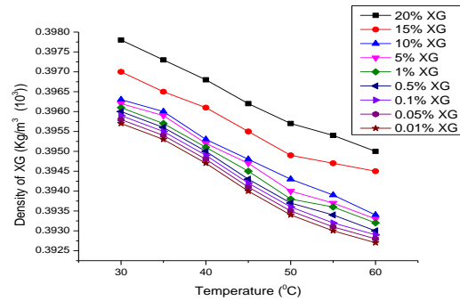
Fig.3.b Effect of temperature on density of XG-Fe mixture
