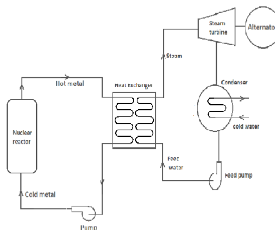
Fig 2: Block diagram of Nuclear power plant
