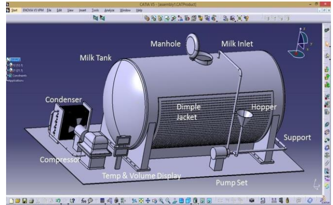
Fig 2.General Arrangement Diagram of Milk chiller Table1 : Component specification
