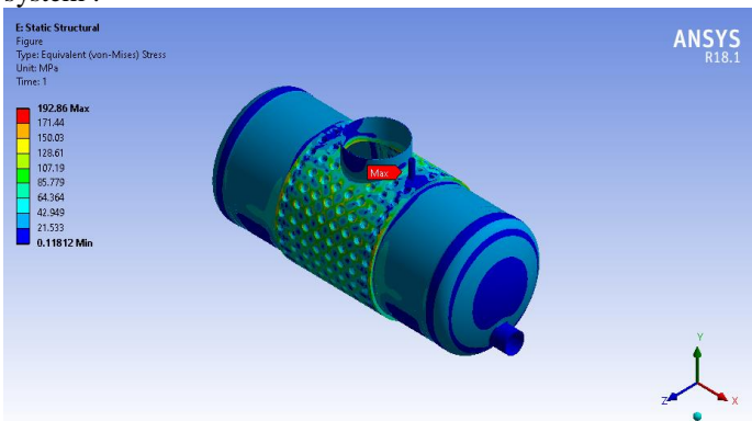
Fig 11 .Resultant Equivalent stress
