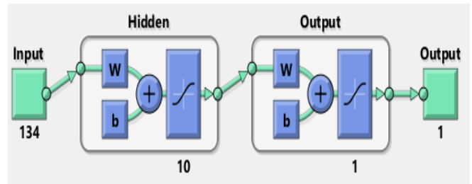
Fig. 6. Architecture of Neural Network
