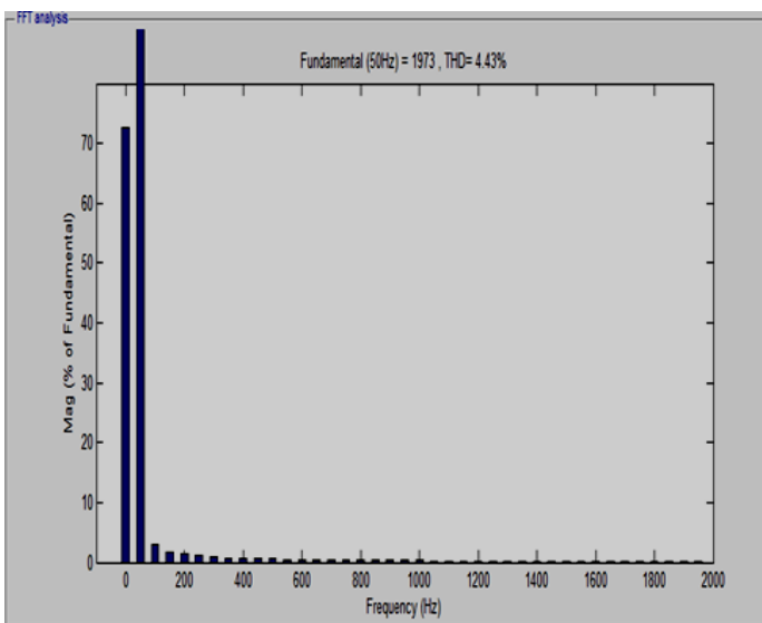
Fig. 10. FFT Analysis
