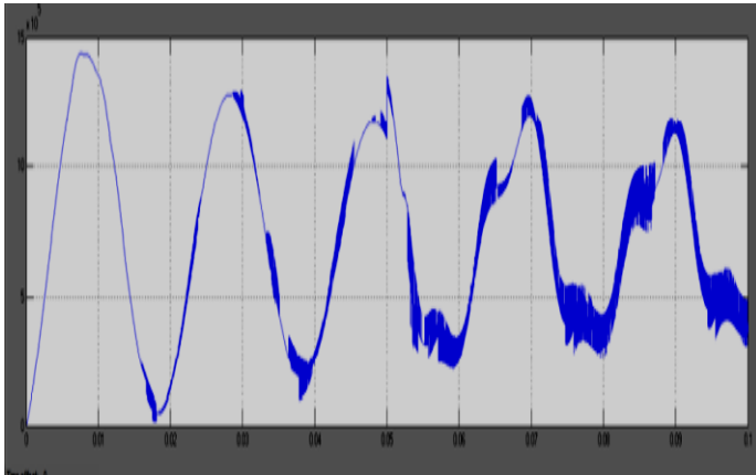
Fig. 9. Reactive power after compensation
