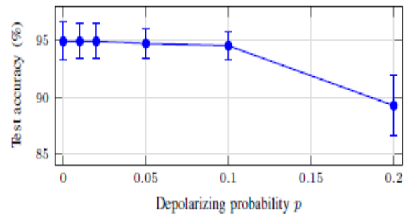
Fig. 3: VQC test accuracy versus depolarizing noise level (mean \pm std over 3 seeds).
