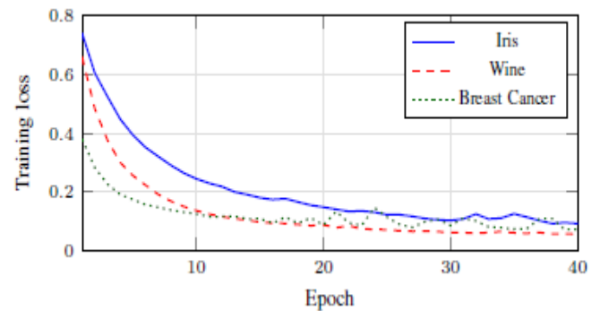
Fig. 2: Mean training loss of the VQC ( n = 4 , L = 3 ) over 40 epochs.
