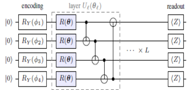
Fig. 1: Variational circuit for n = 4 qubits: angle encoding, L repeated layers of general rotations and a CNOT ring, and Pauli-Z readout.
