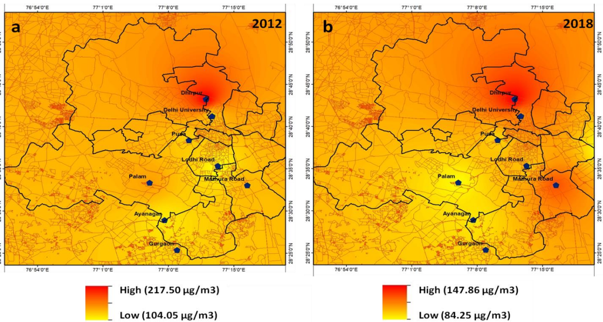
Fig.3: Stationwise spatial changes of PM 2.5 in 2012(a) and 2018(b)
