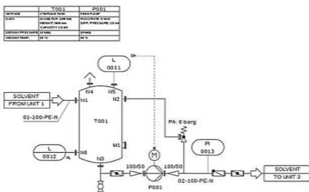
Figure 5 the Instrumentation Part of a Piping and Instrumentation Diagram
