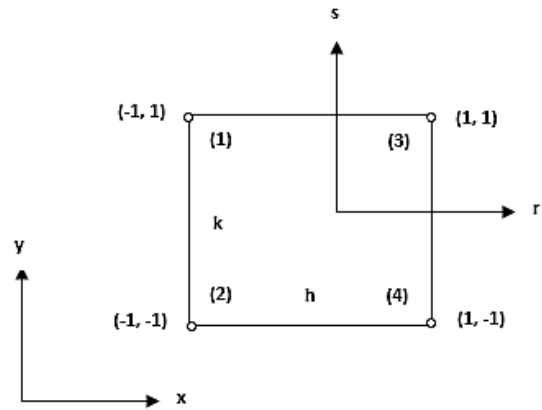
Fig. 3. 4 – Noded element
