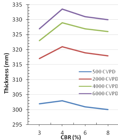
Fig. 3 Effect of CBR on Thickness of Rigid Pavement
