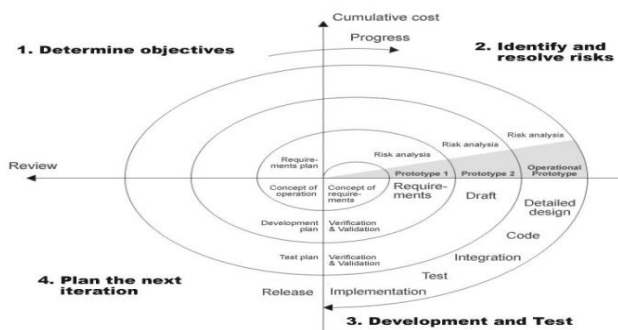
Figure 1. Methodology
