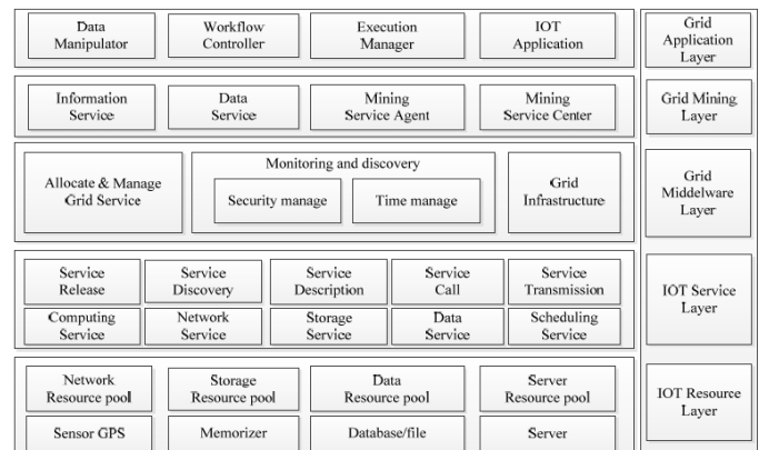
Fig.5 Grid based Data mining Model
