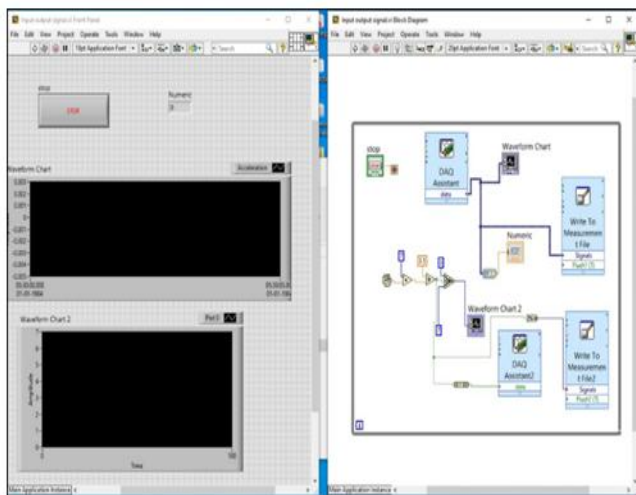
Fig. 3. LabVIEW interface and block diagram for input-output data acquisition.
