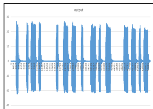
Fig. 9. Mild-steel output data (Acceleration vs time)
