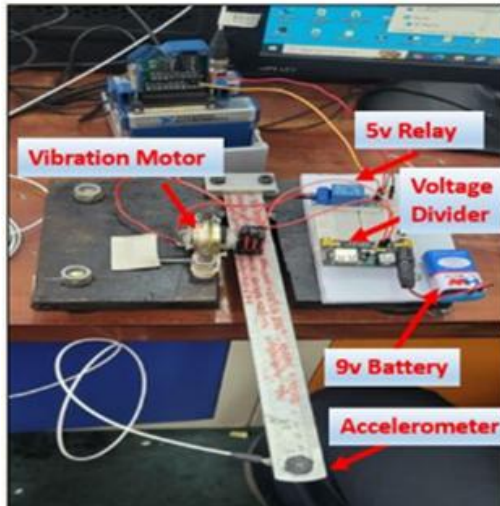
Fig. 2. testing setup
