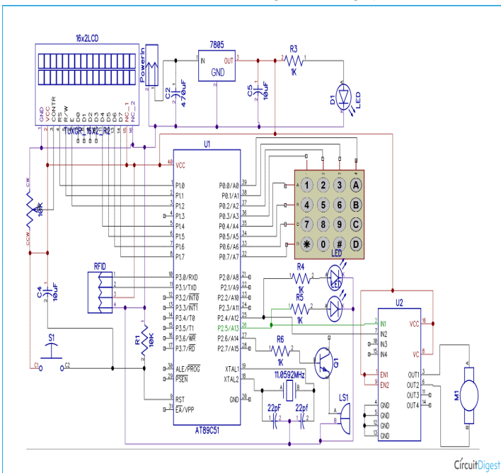
Fig 8 RFID based e-passport schematic
