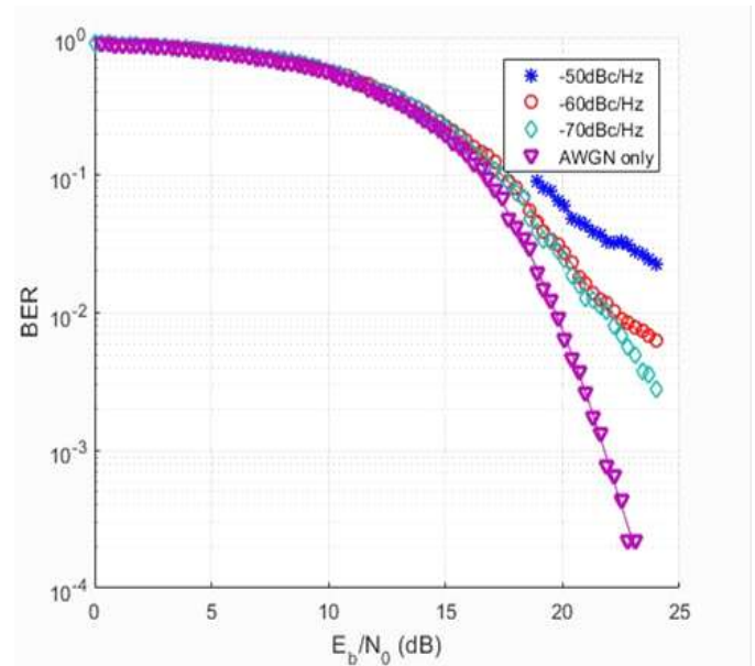
Figure 6.6: BER vs. E_b/N_0 for 128 QAM at different phase noise level densities and without the presence of phase noise.
