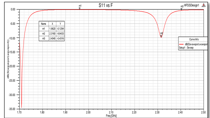
Fig.11: Plot of reflection coefficient ( S_{11} ) vs. frequency for rectangular patch micro strip antenna, S_{11} (dB) on y-axis, frequency (GHz) on x axis at frequency 2.3GHz
