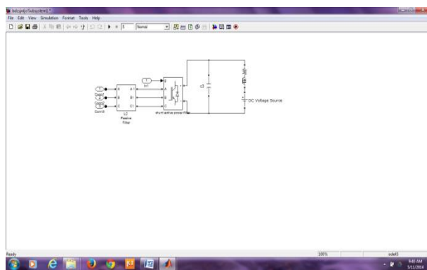
Fig 9. Design shunt active filter
