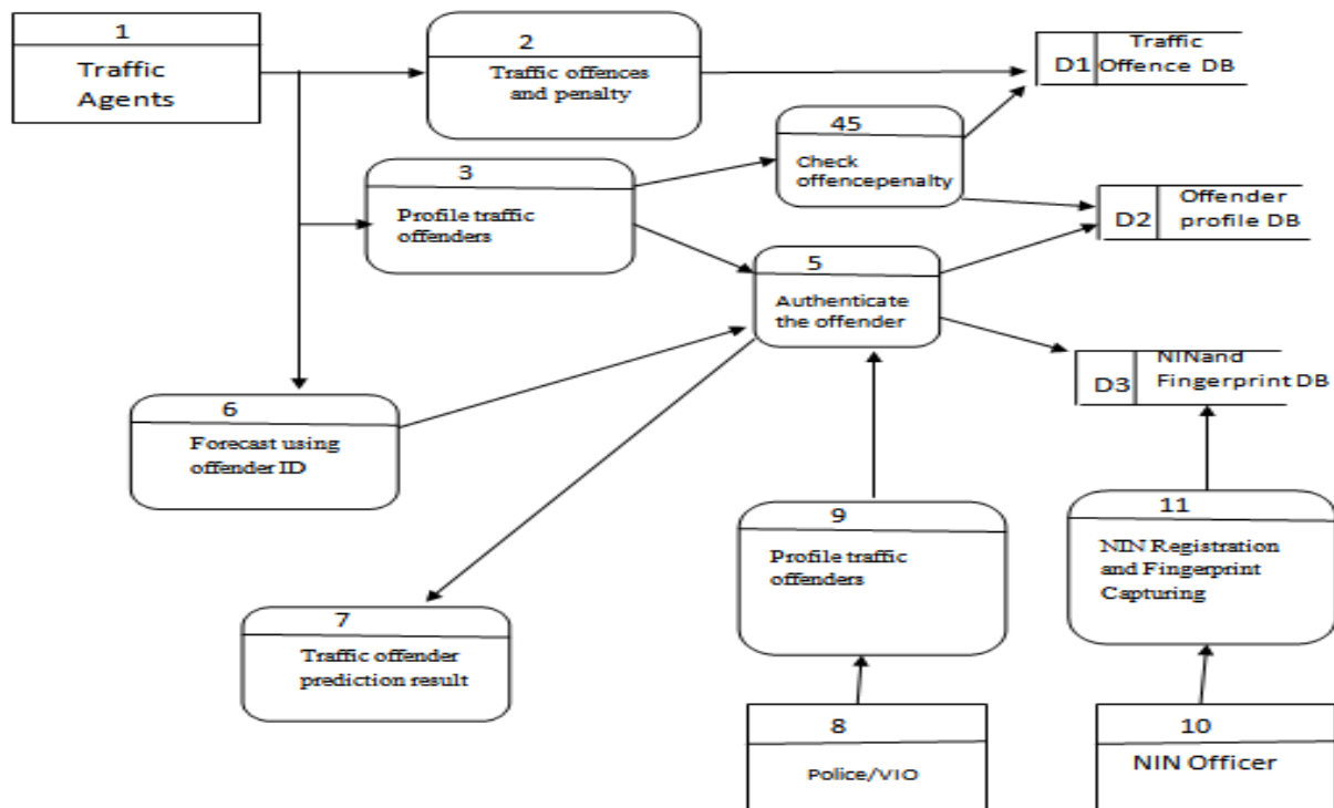
Figure 4: Data Flow Diagram of the proposed system
