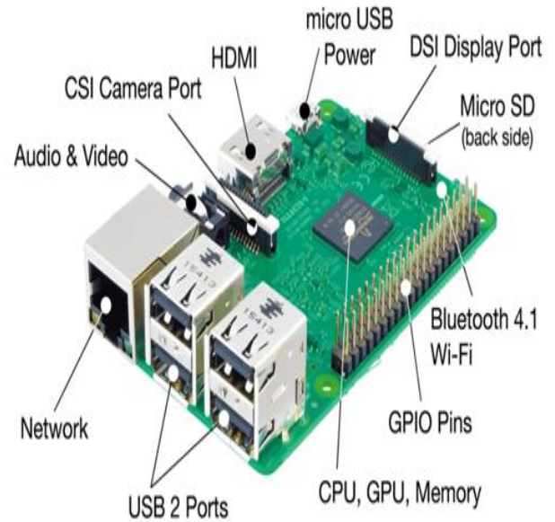
Raspberry Pi-3 Model B
