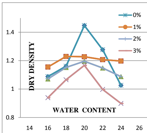
Graph 3.1 Compaction Test Result for Black Cotton Soil with Corchorus capsularis Fiber
