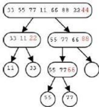
Fig. 3. Shows the partitioning of the input array into single element arrays. The red element is the pivot element of the array.
