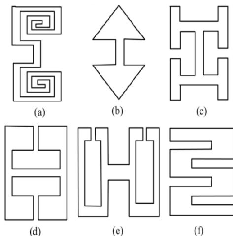
Fig1: Different shapes of Defeated Ground Structure (DGS)
