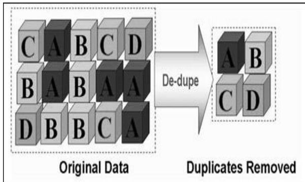
Fig. 2. Data De-duplication[12]
