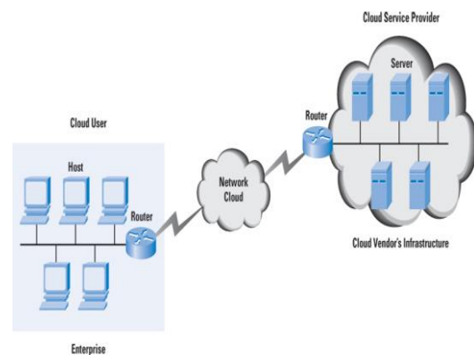
Fig. 1. Cloud Computing[11]
