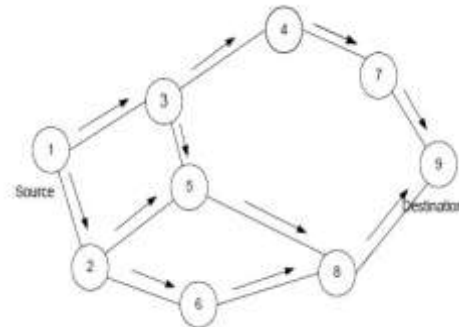
Fig. 1.2.The Route Request Packets Flooding in AODV
