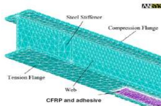
Figure 20: 3D simulated specimen (Narmashiri K. et al. (2001) [37]).
