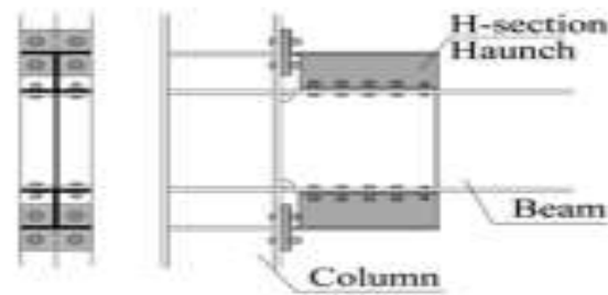
Figure 1. Proposal for seismic retrofit by supplemental H section haunches (Hayato Asada et al.2014 [27]).
