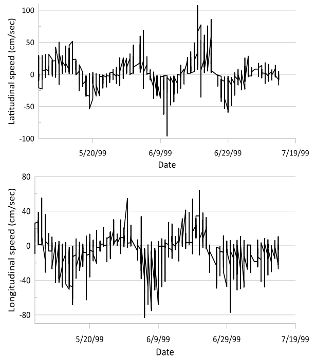
Figure (8) Latitudinal and longitudinal speed inferred from drogue 3745 tracks
