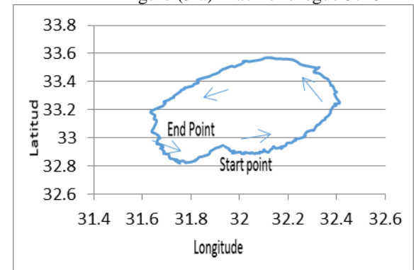
Figure (5-b) Track of one complete gyre
