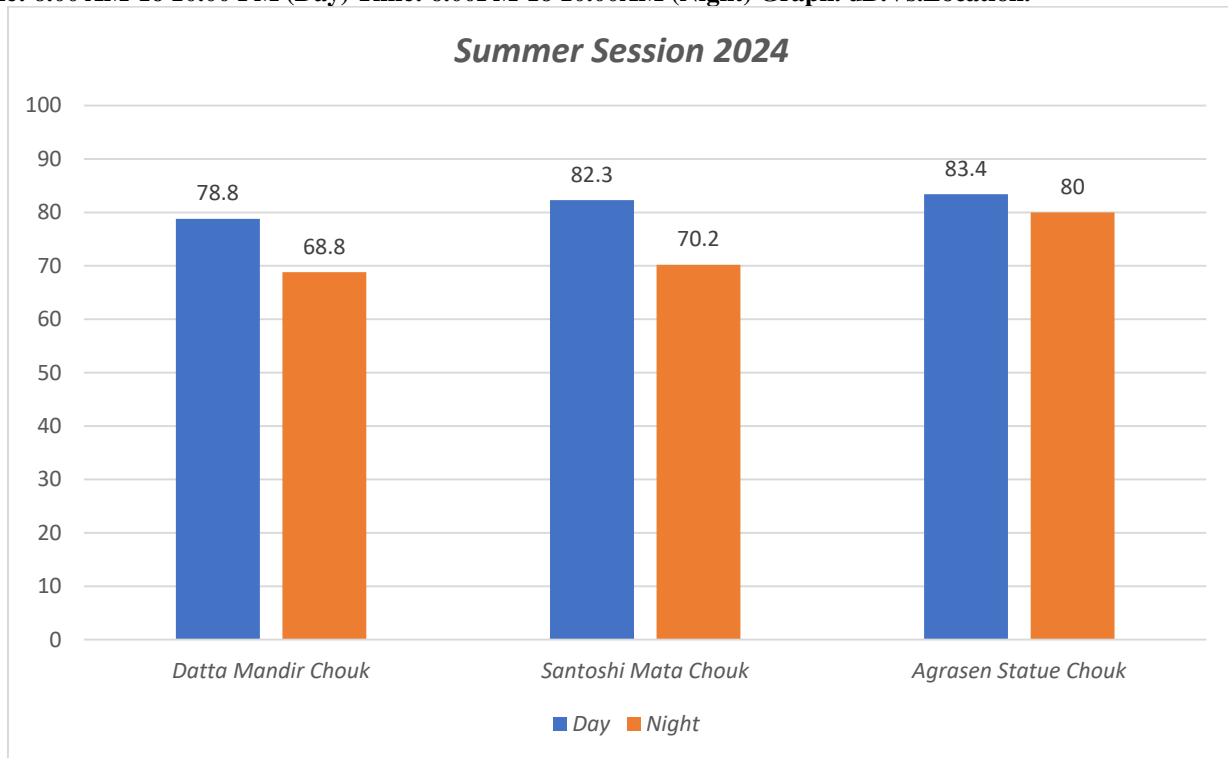
B] Time: 6.00 AM To 10.00 PM (Day) Time: 6.00PM To 10.00AM (Night) Graph. dB.Vs.Location.
