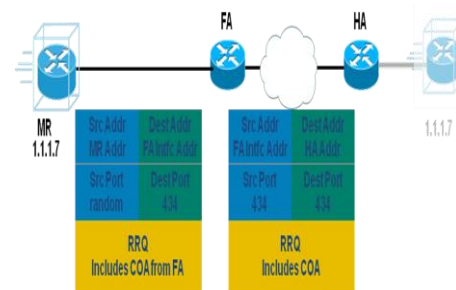
Fig.4. Sending RRQ
