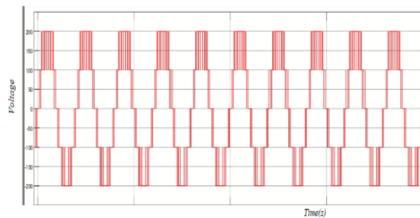
Figure 8: single phase voltage of five level inverter
