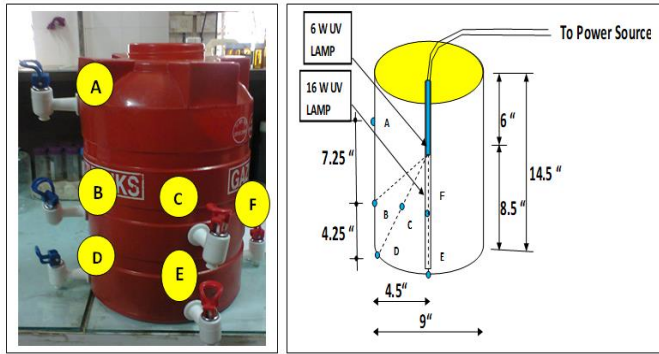
Figure 6: 15 Liter Water Tank with Sample Collection Port
