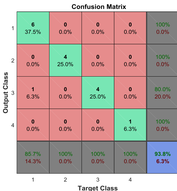
Fig. 2 Confusion matrix of the proposed model for 4-class classification
