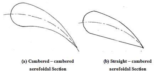
Fig. 3. Two Types of Aerofoil Section Profiles
