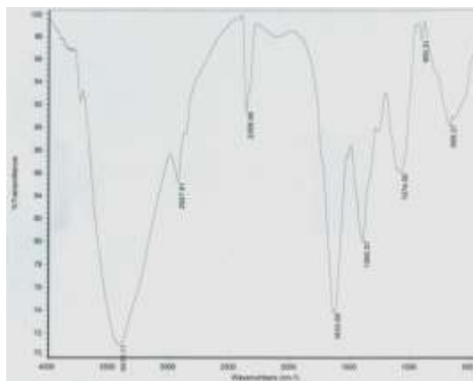
Fig 5. FT-IR spectrum of Ag nanoparticles
