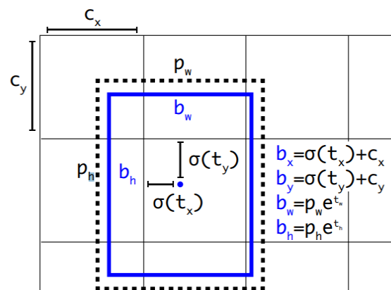
Fig. 2. Diagram representing the working of Bounding boxes
