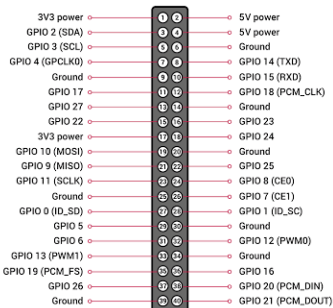
Fig. 2. GPIO-Raspberry Pi
