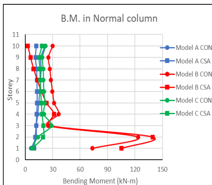
Fig. 10. B.M. in Normal columns
