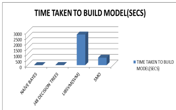
Fig 4. A Graph of Different types of Algorithm as against time taken to build the model (secs) for 25 attributes
