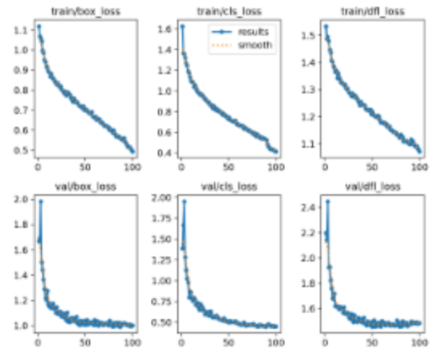
Fig. 4. Loss graph for training and validation dataset.
