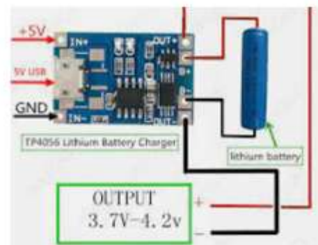
Fig. 4. TP4056 charging circuit with 3.7v Li-Po Battery
