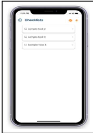
Figure 9. Checklist Dashboard
