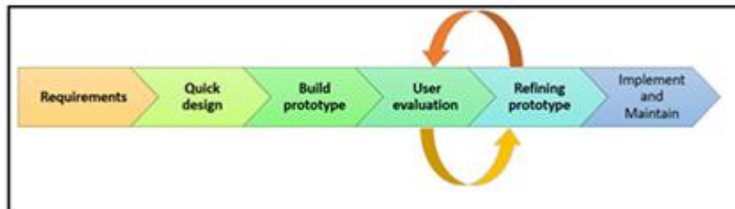
Figure 3. Prototyping Model
