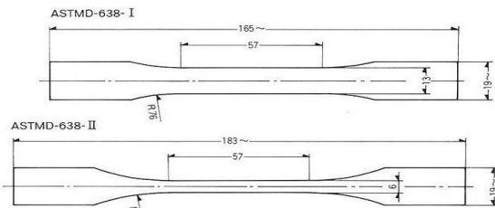
FIGURE 2. ASTM 638 - I & II standard size.
