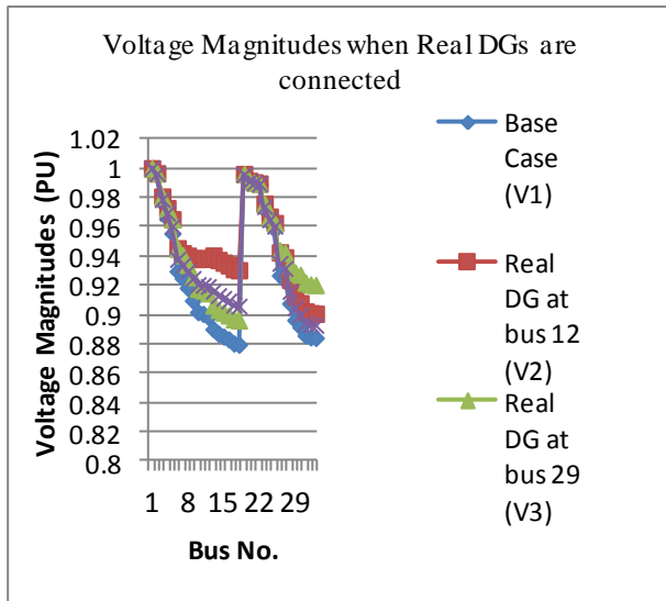
Fig. 3. Voltage comparison when real DG is connected
