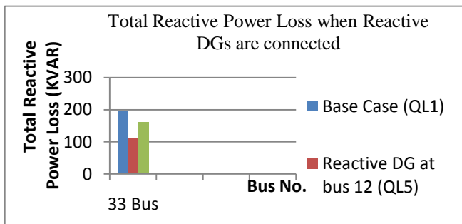
Fig. 8 Reactive power loss comparison when reactive DG is connected
