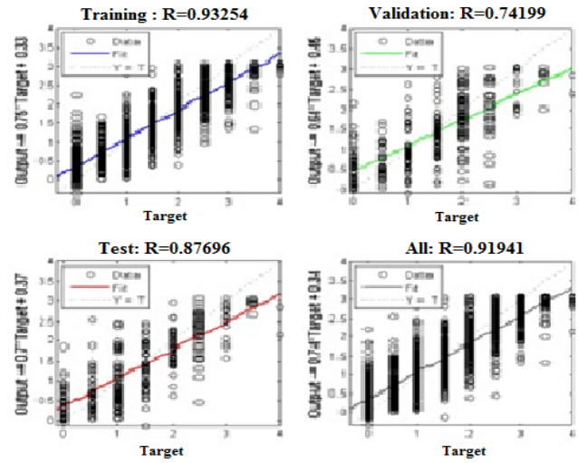
Figure 1.7 Using different datasets for implementation of the system at different circumstances and combining them and checking both of there test as well as train accuracies.
