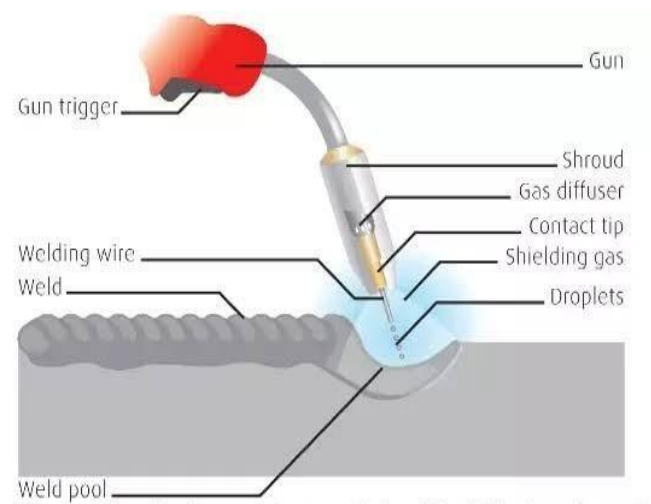
Fig. 1. Fusion Type Welding
