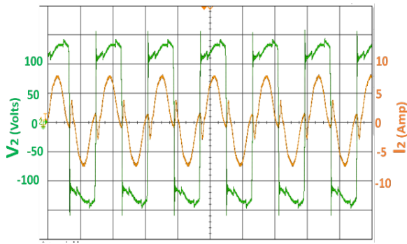
Fig. 7. Experimental waveforms (a) Inverter switching pulses, (b) Inverter output voltage and current, (c) Receiver output voltage and current.
