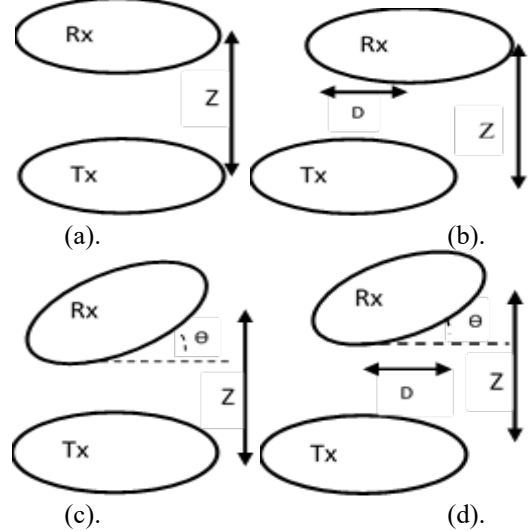
Fig. 3. Possible alignments of Tx and Rx Circular Coils (a) Perfect Alignment, (b) Lateral Misalignment, (c) Angular Misalignment, (d) Lateral and Angular Misalignment.
