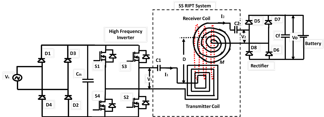
Fig. 1. Schematic diagram of inductive power transfer system.
