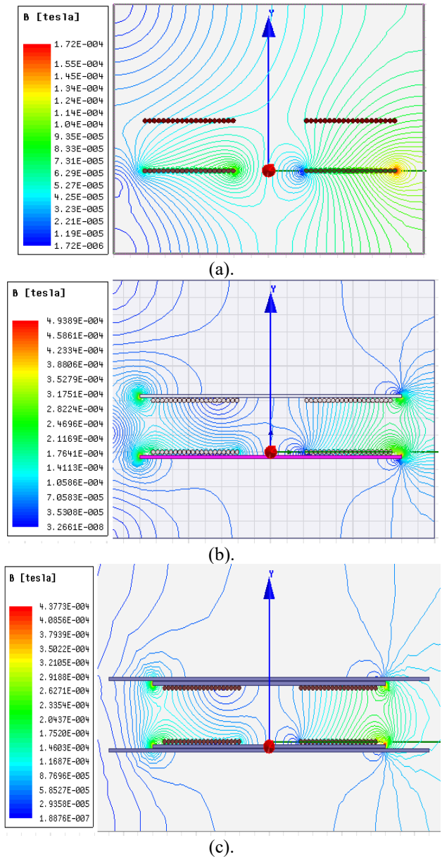
Fig. 5. 2-D (a) Magnetic flux density distribution between connected coils' Perfect Alignment at 100mm distance. Square-Circle ohne Kern (b). Cored square-circle. Short square-circle with core and chassis.
