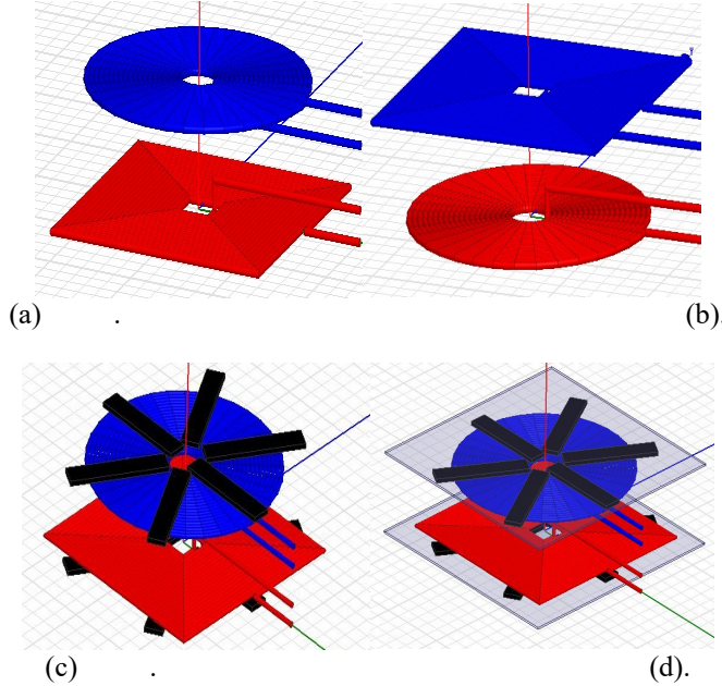
Fig. 4. FEM interoperability coils. Square-Circle (b). Circle-Square. Cored square-circle. Short square-circle with core and chassis.
