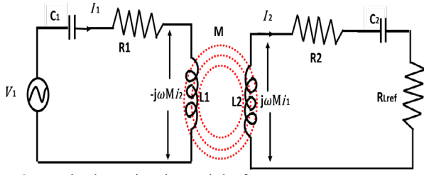
Fig. 2. Equivalent circuit model of SS resonant IPT system.
